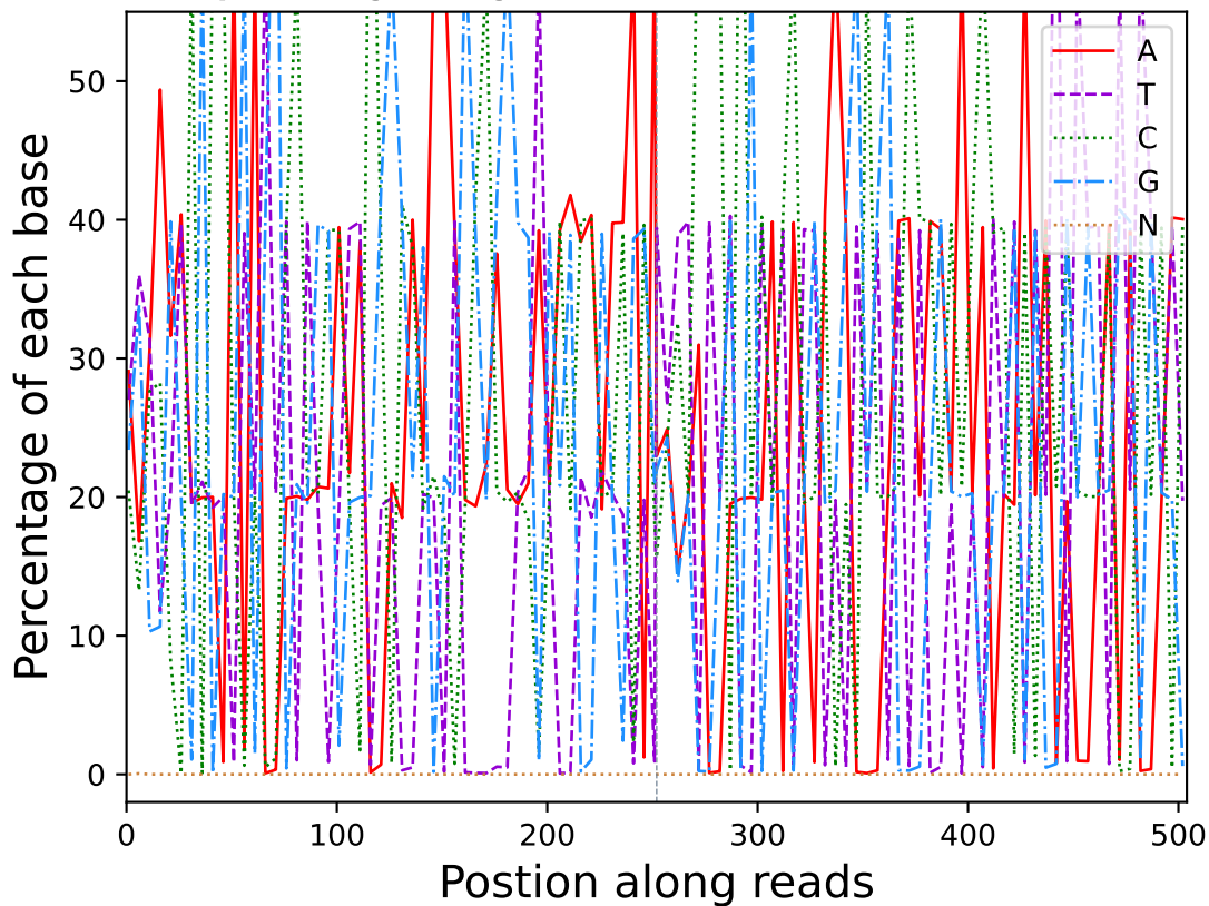
Base percentage along reads (R10708)
